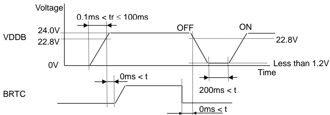
Figure 5.4.1 Backlight on/off
