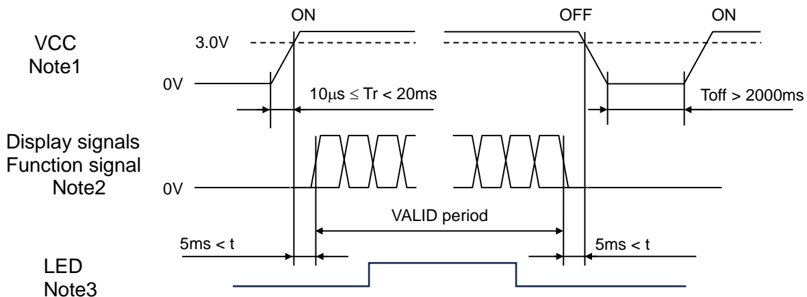
Figure 5.3 Power on/off sequence
