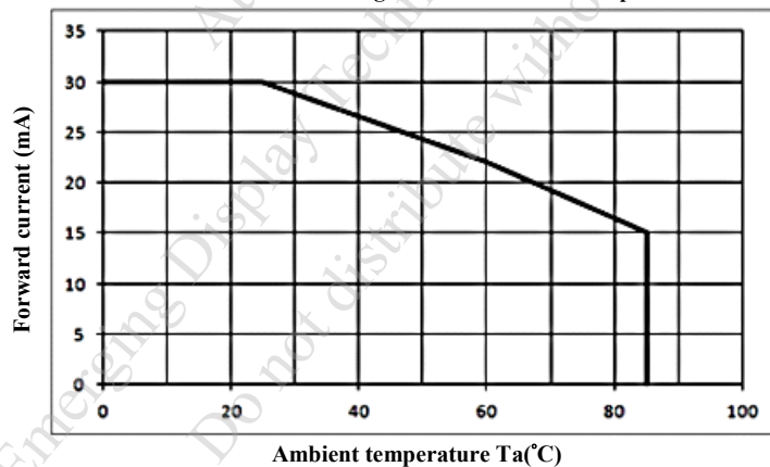
Forward current derating curve VS.Ambient temperature
