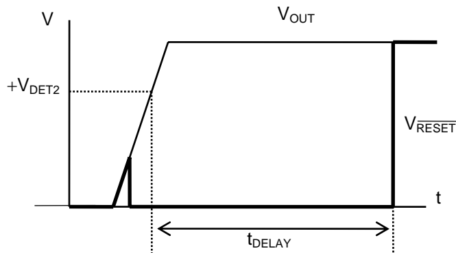
Figure 7 Definition of \overline{\text{RESET}} Release Delay Time ( t_{\text{DELAY}} )
